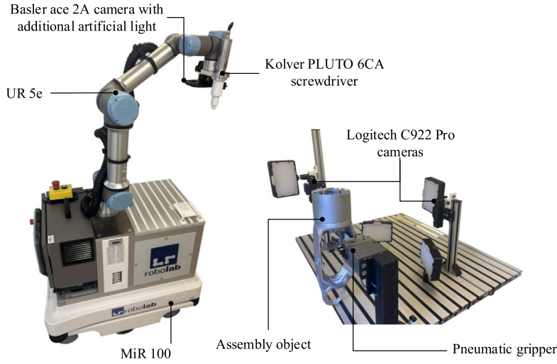
Fig. 1. Overview of the components of the proposed system used for addressing the screwdriving problem through mobile manipulation. On the left side of the figure is the mobile manipulation system, consisting of a MiR100 mobile platform upgraded with a collaborative UR 5e manipulator. The manipulator is equipped with a Kolver PLUTO 6CA industrial screwdriver, a Basler ace 2 A camera, and a Wenglor LRLW100 ring-shaped LED light. On the right side, the workstation components are presented, comprising two Logitech C922 Pro RGB cameras, LED panel lights, and a pneumatic gripper holding the assembly object.
